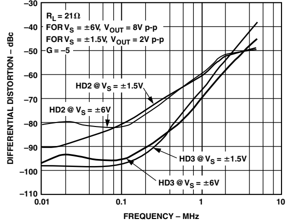
TPC 22. Differential Distortion vs. Frequency
